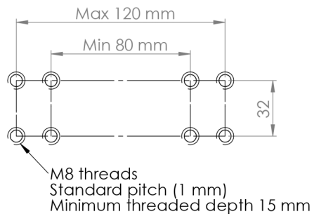
TYPE 2: Four M8 holes in triple clamp
