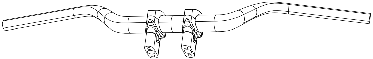
TYPE 2: Four M8 holes in triple clamp
