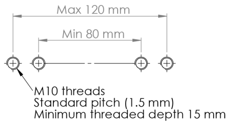
TYPE 1: Two M10 holes in triple clamp
